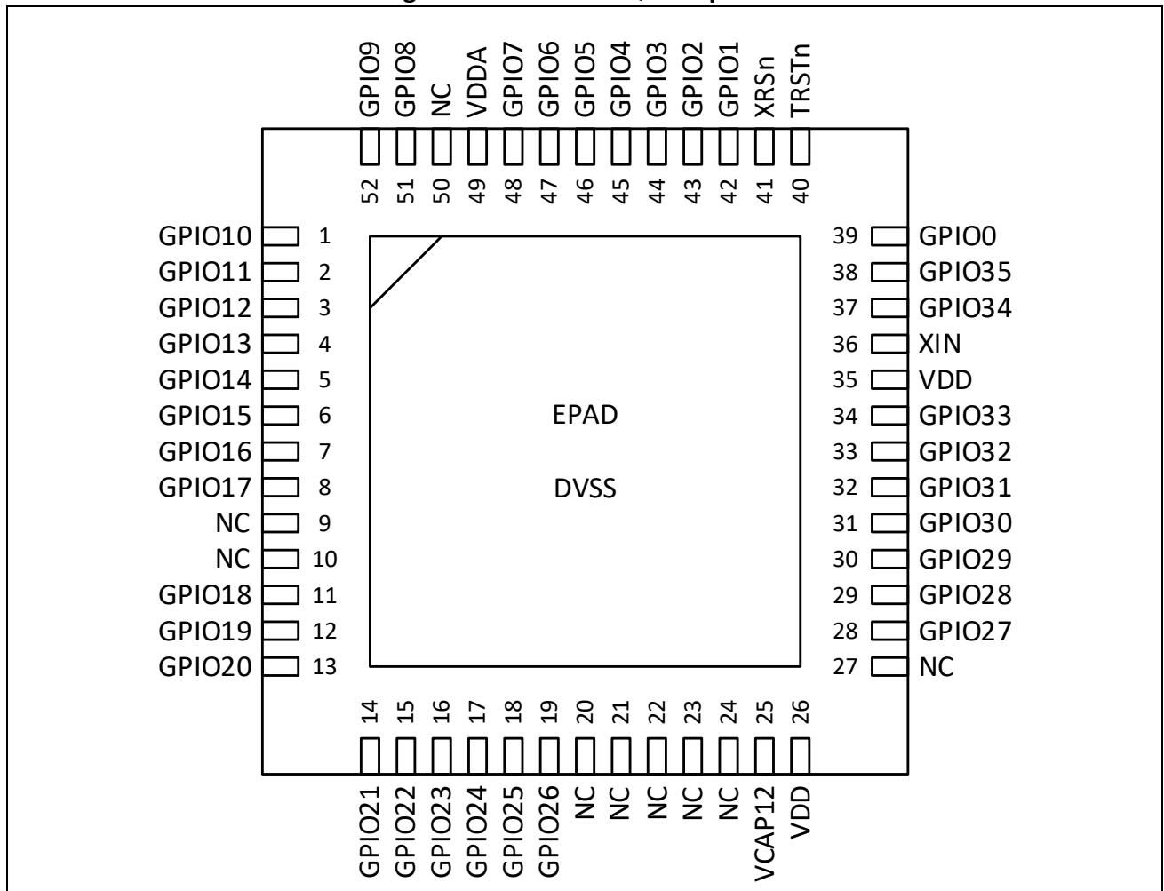
Figure 3-2: SPC1068 QFN52 pinout
