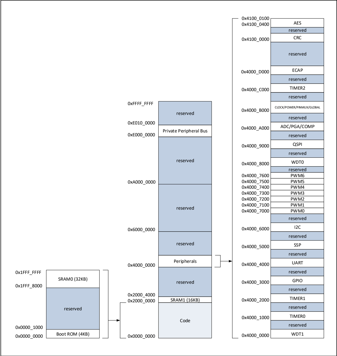
Figure 4-1: Memory map
