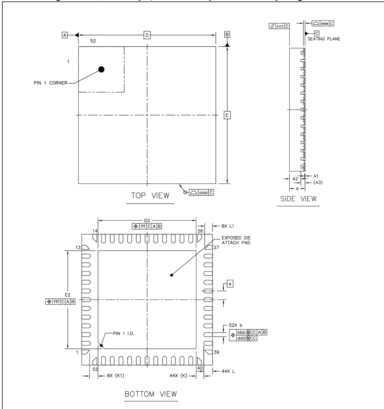
Figure 6-3: QFN52 - 52 pin, 6mm x 6mm quad flat no-lead package outline
