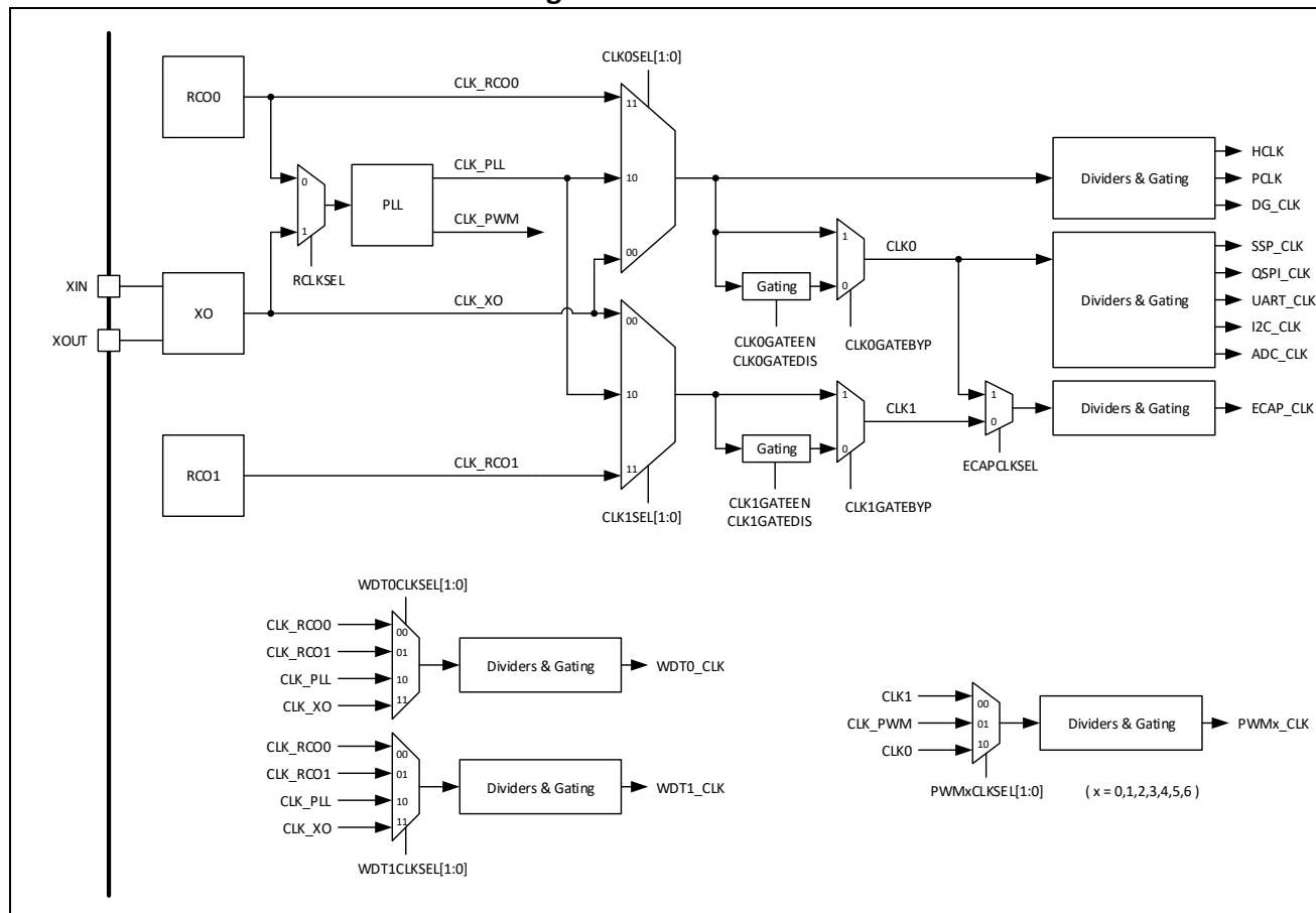
Figure 1-2: Clock tree
