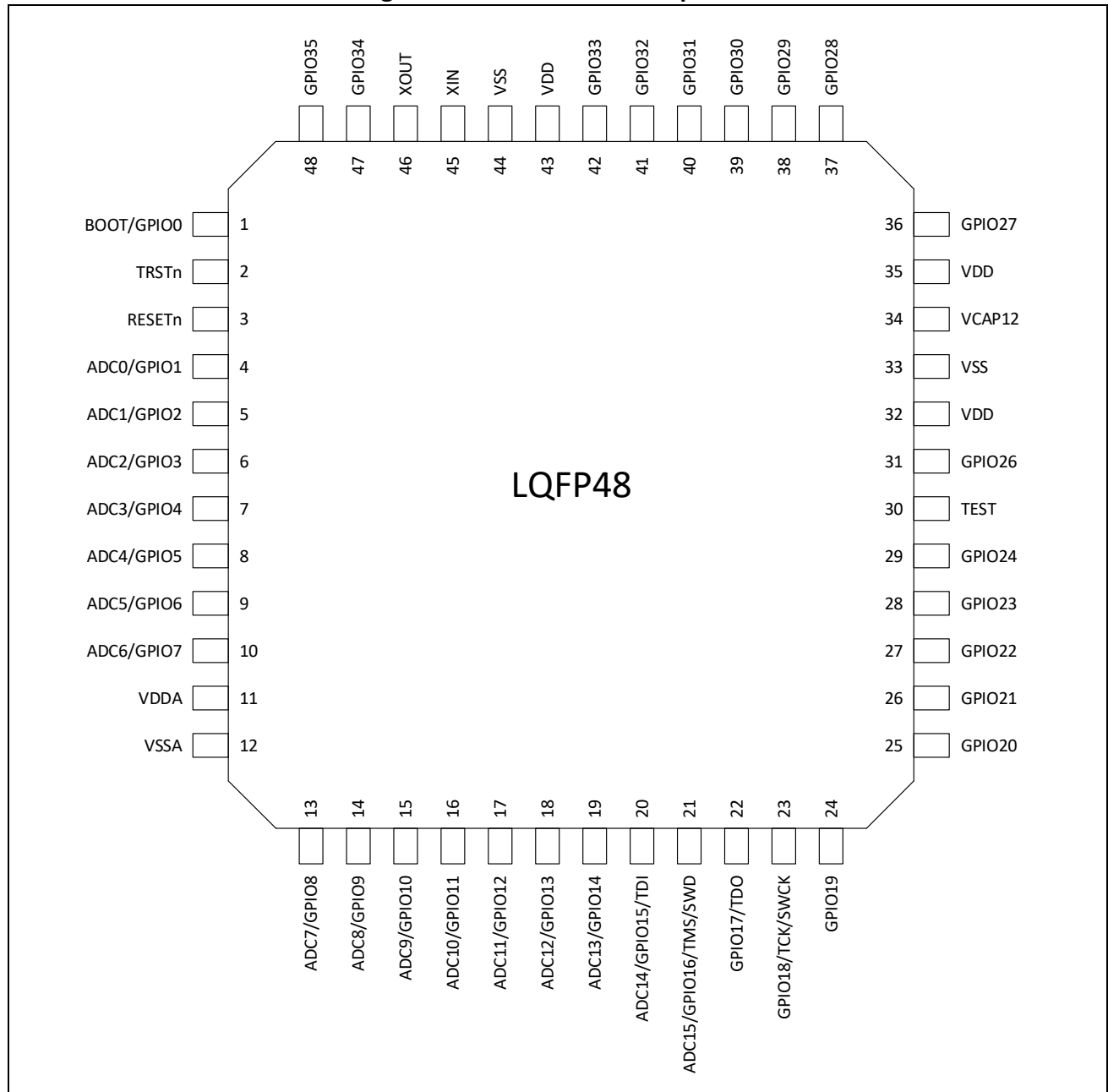
Figure 3-1: SPC1068 LQFP48 pinout
