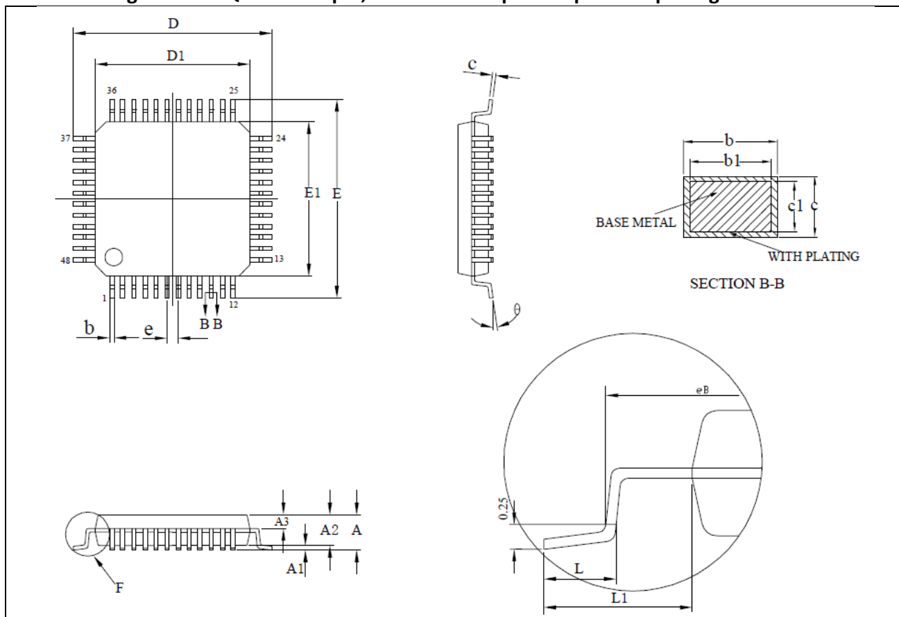
Figure 6-1: LQFP48 – 48 pin, 7 x 7 mm low-profile quad flat package outline
